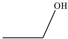
Figur 1: Ethanol structure
